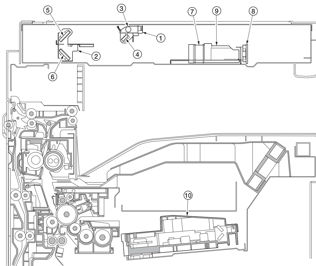
Figure 2-1-7 Optical section
