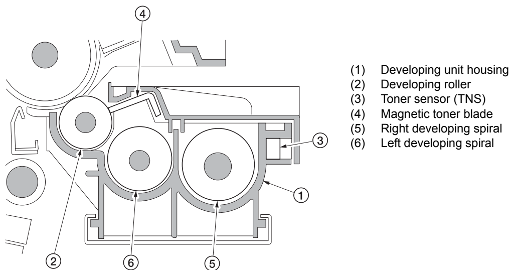
Figure 2-1-13 Developing section
