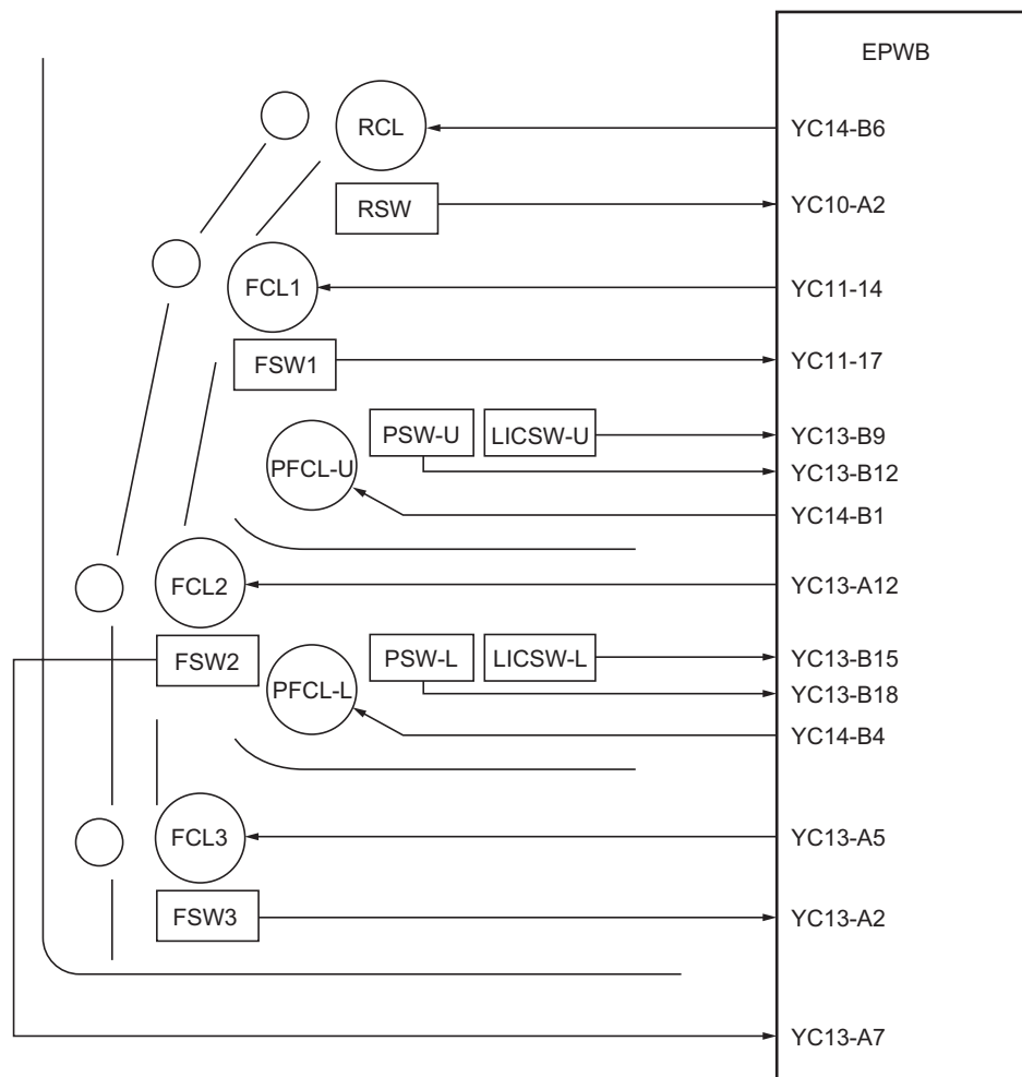
Figure 2-1-3 Paper feed section block diagram (cassettes 1 and 2)
