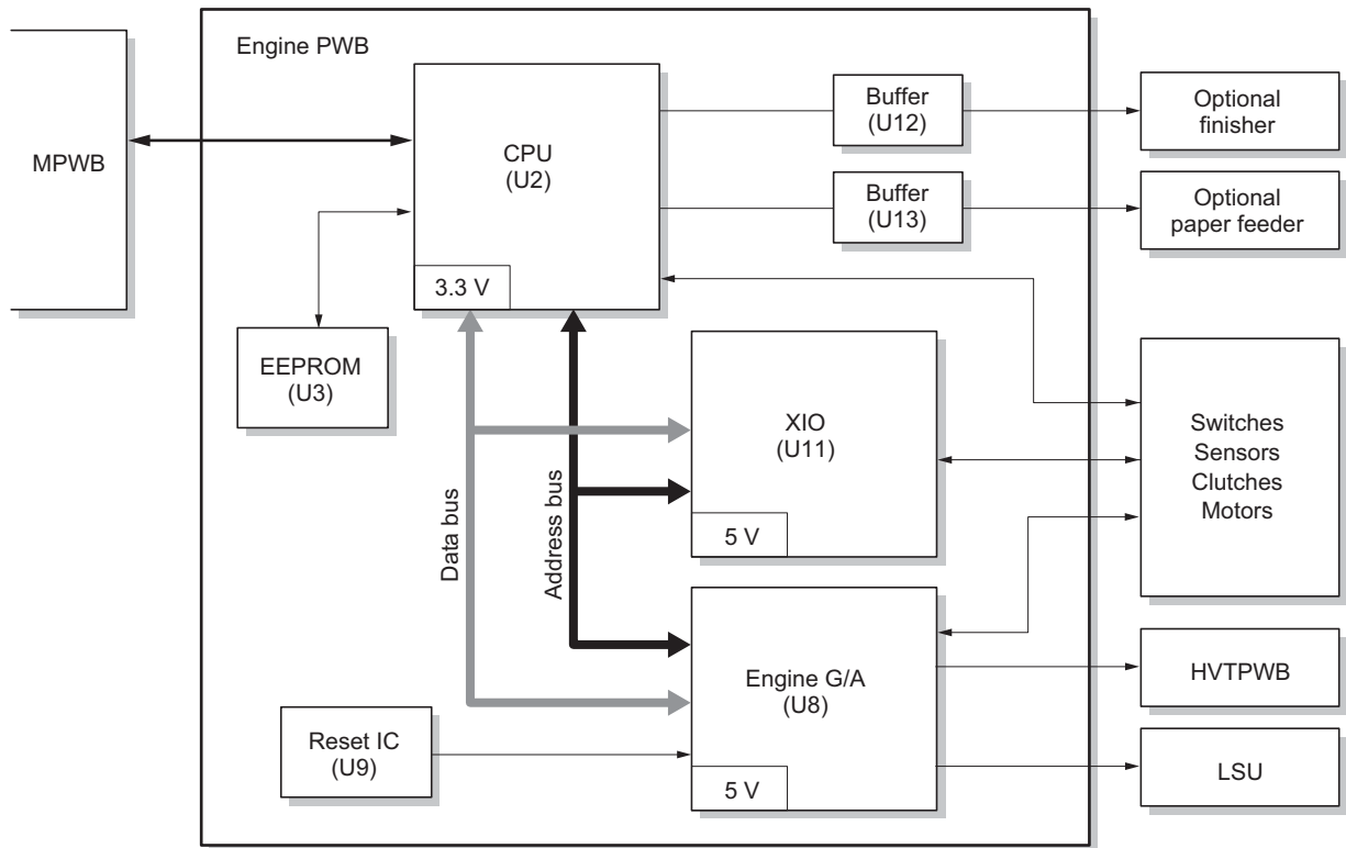
Figure 2-3-3 Engine PWB diagram
