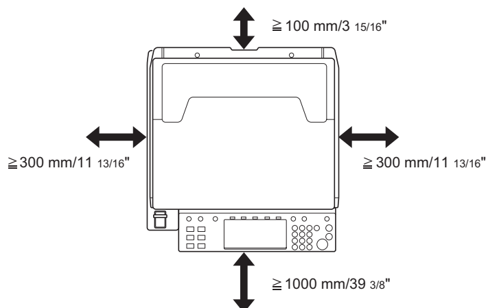
Figure 1-2-1 Installation dimensions
